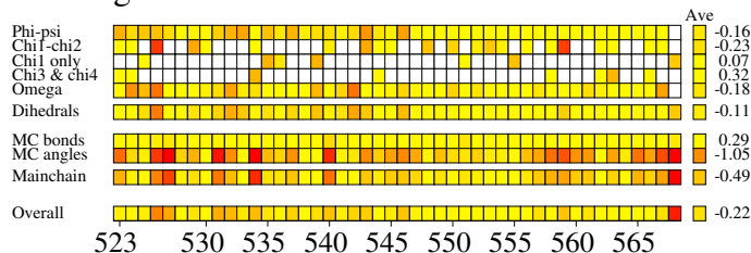
g. G-factors
