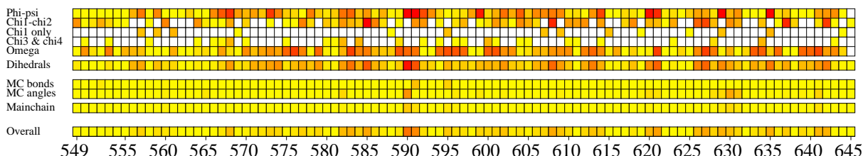
g. G-factors
