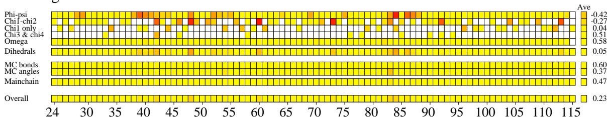
g. G-factors
