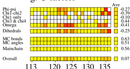
g. G-factors
