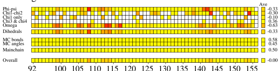
g. G-factors
