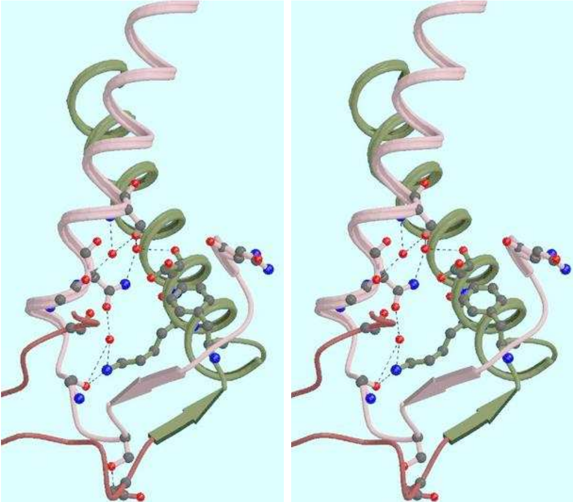
Figure 5 Superset: Antimycin Binding Site in Cytochrome bc 1 . See legend to Figure 5 for explanation. This set for cross-eyed viewing.
